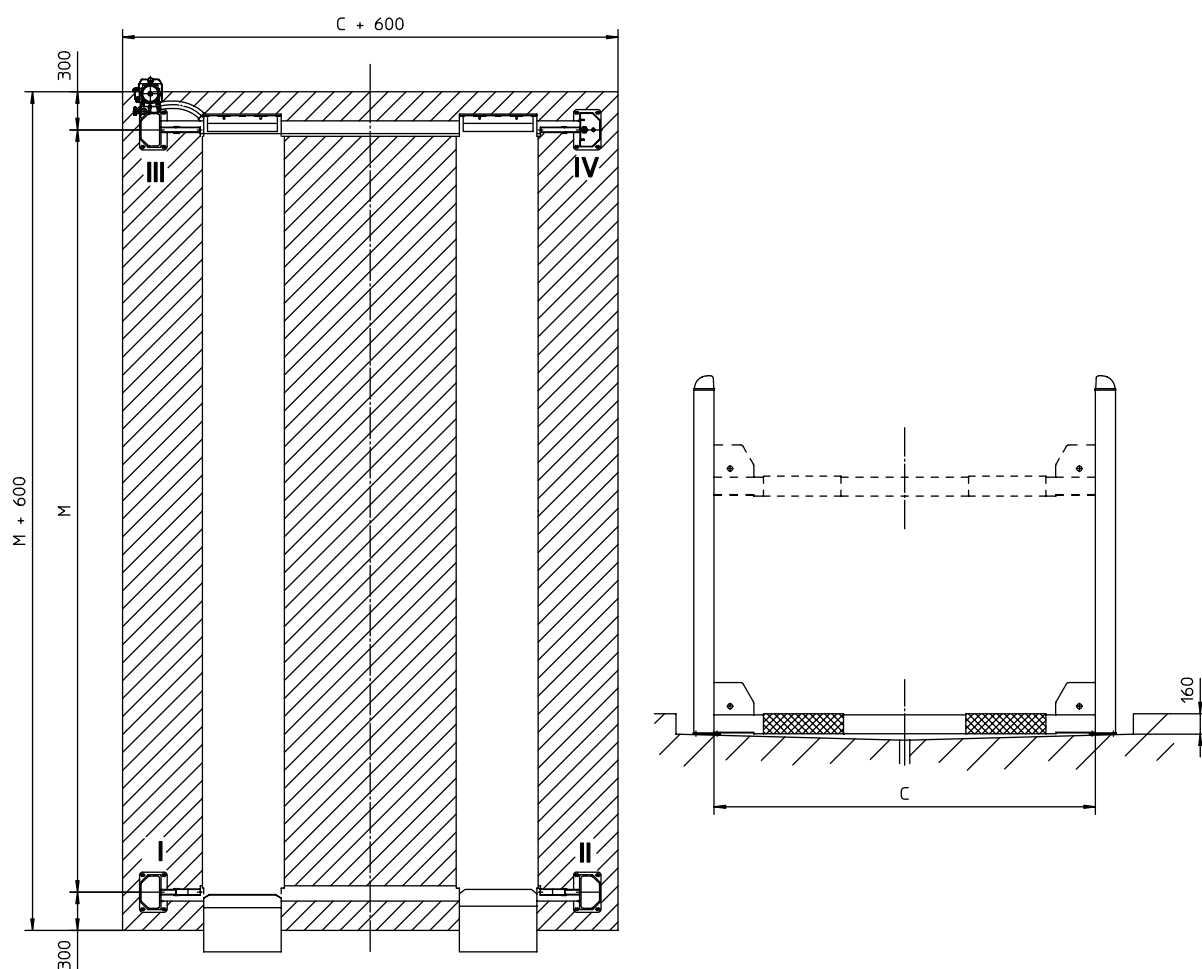
Figure 1.16 Dimensions pit
