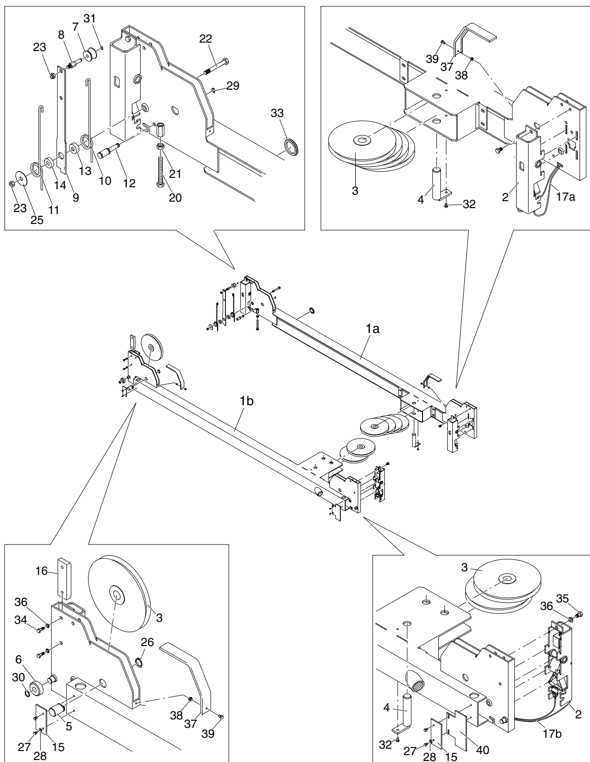
Figure 1.4 Cross beams
