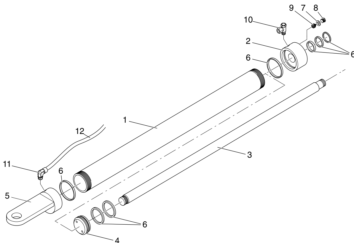
Figure 1.2 Cylinder
