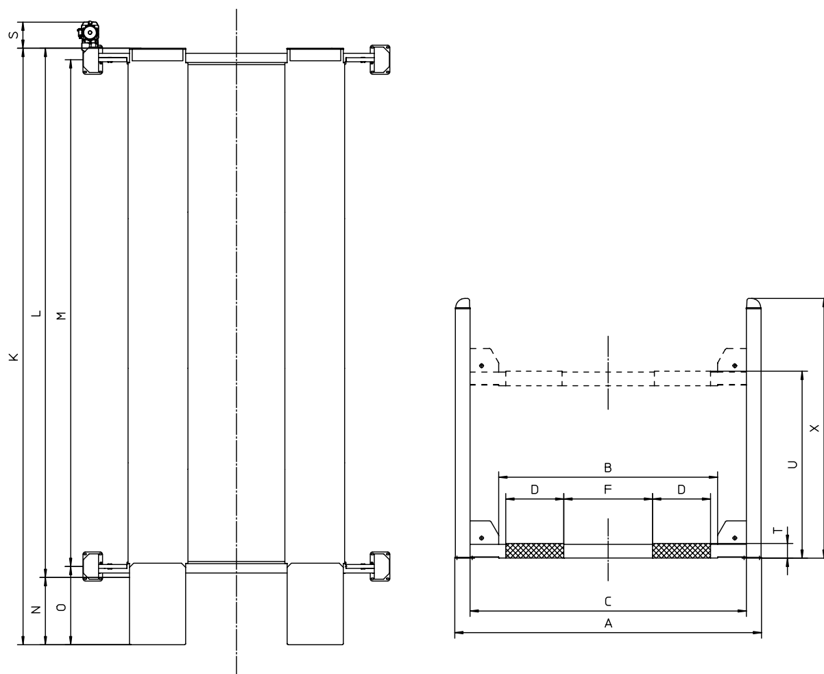
Figure 1.15 Dimensions
