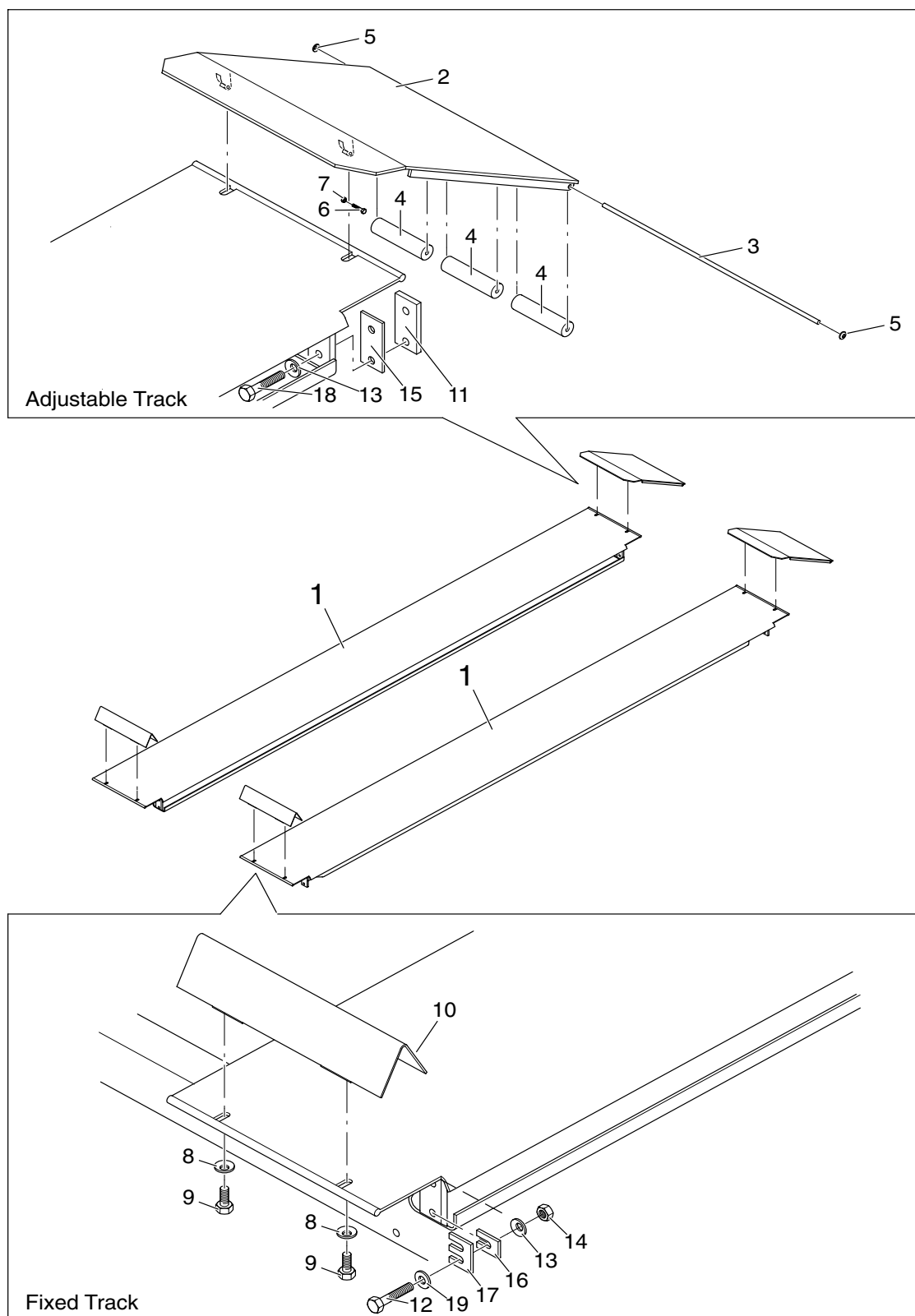
Figure 1.3 Tracks
