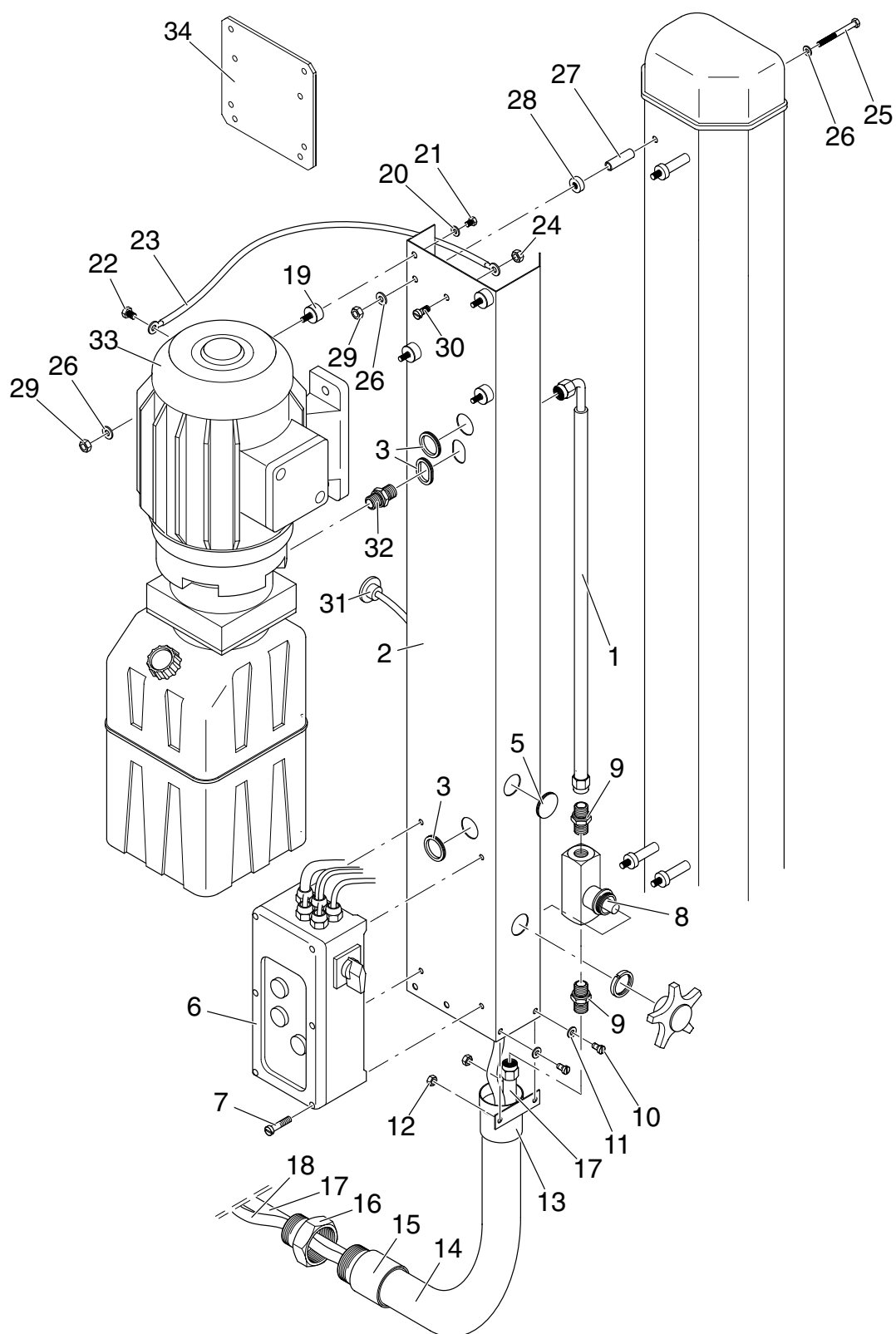
Figure 1.5 Post with operation devices
