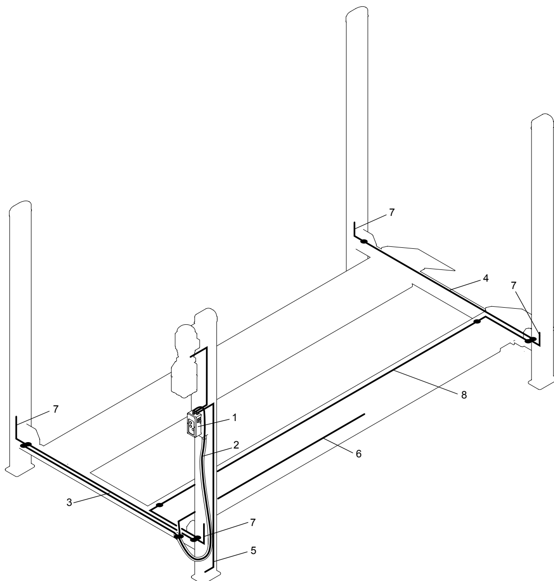
Figure 1.10 Electric cables
