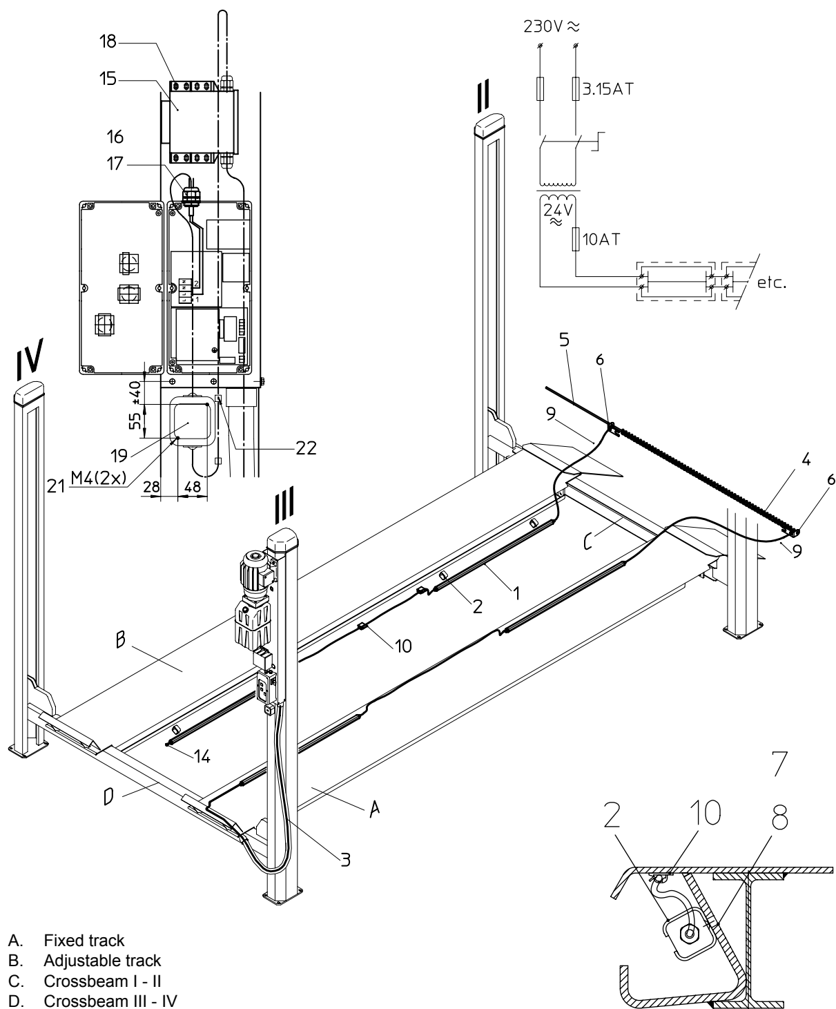
Figure 1.14 Lighting
