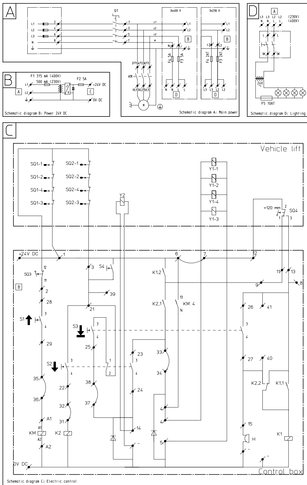
Figure 1.8 Schematic diagram
