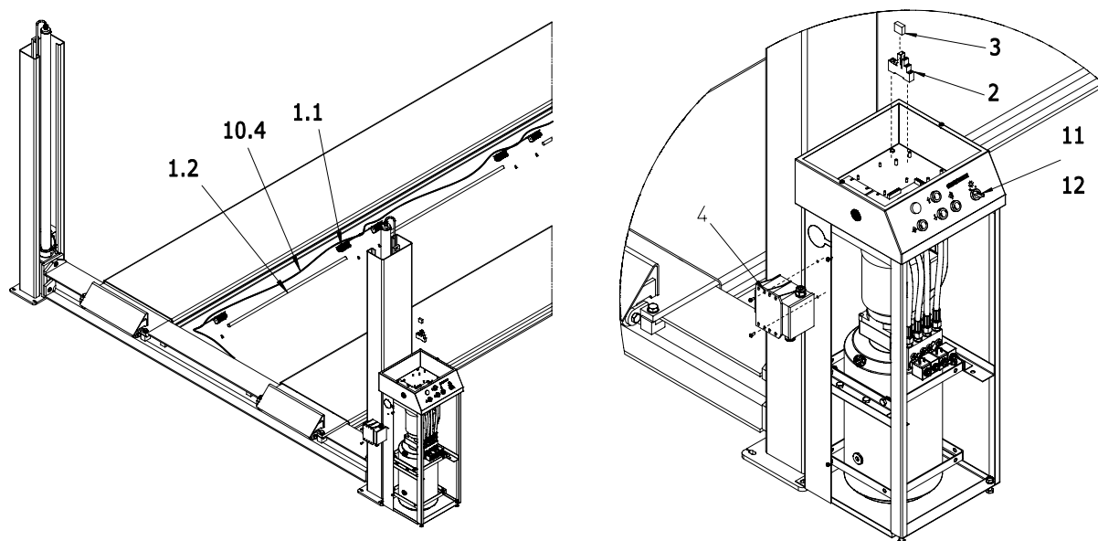
Figure B 1.1 Track lighting (2)
