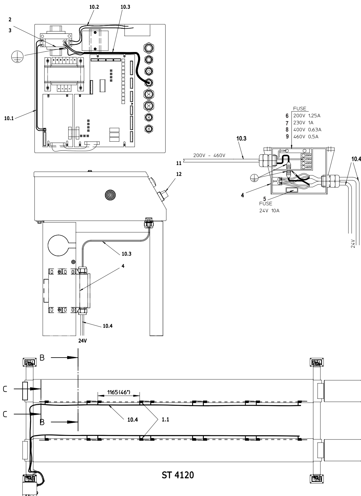
Figure B 1.1 Track lighting (1)
