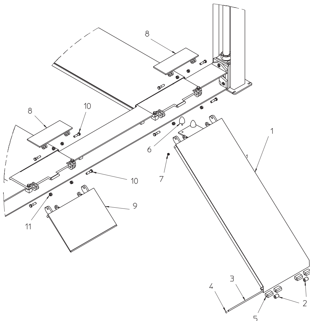
Figure B 2.1 Special drive-on ramps
