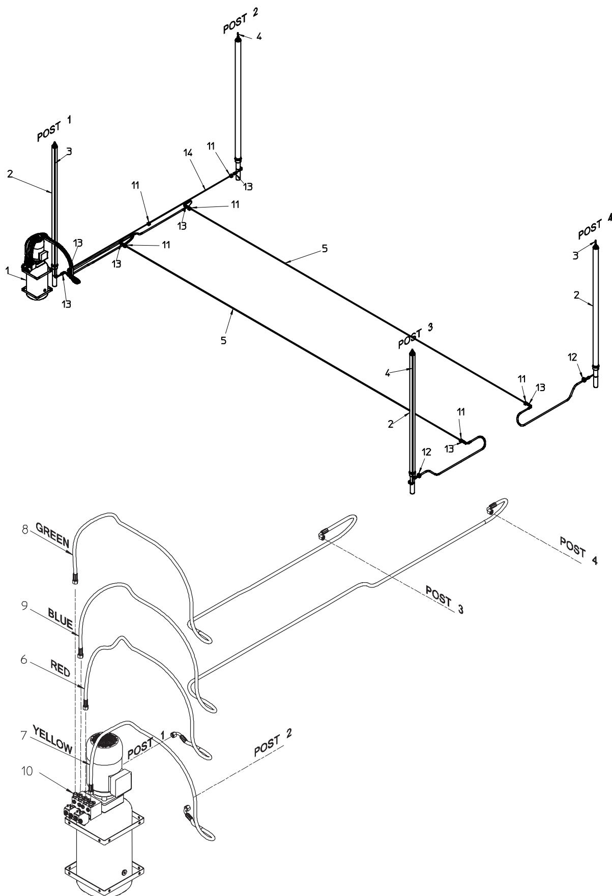
Figure A 4.1 Hydraulic components (1)
