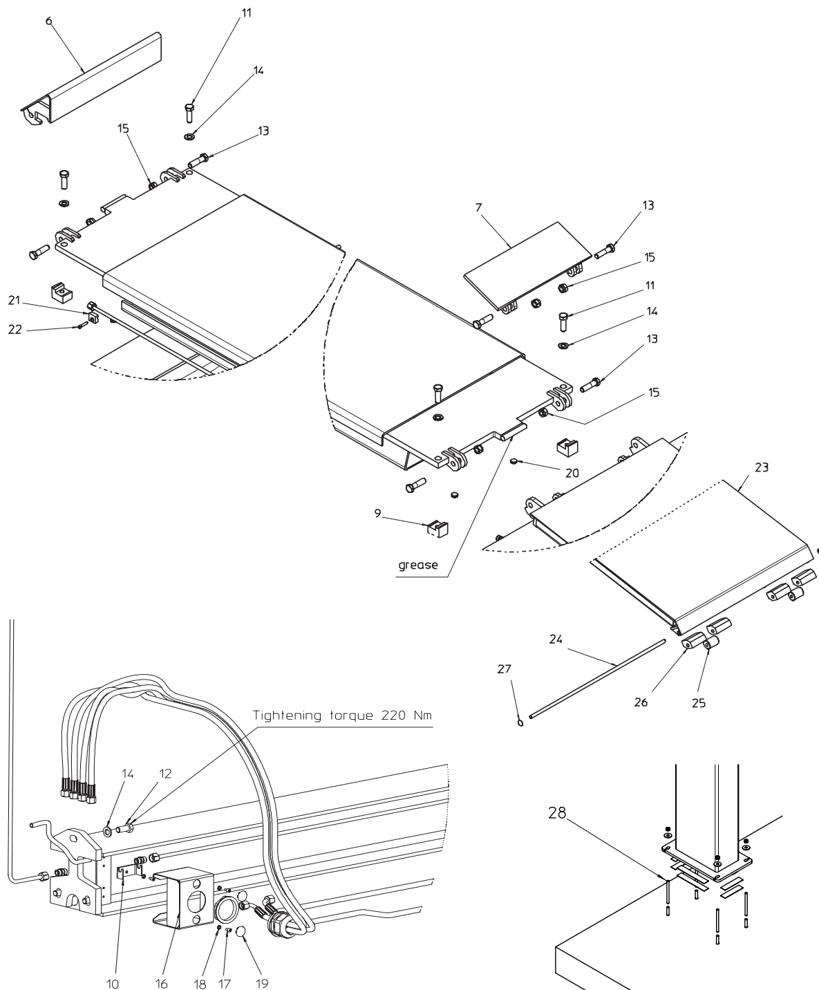
Figure A 1.2 Summary vehicle lift (2)
