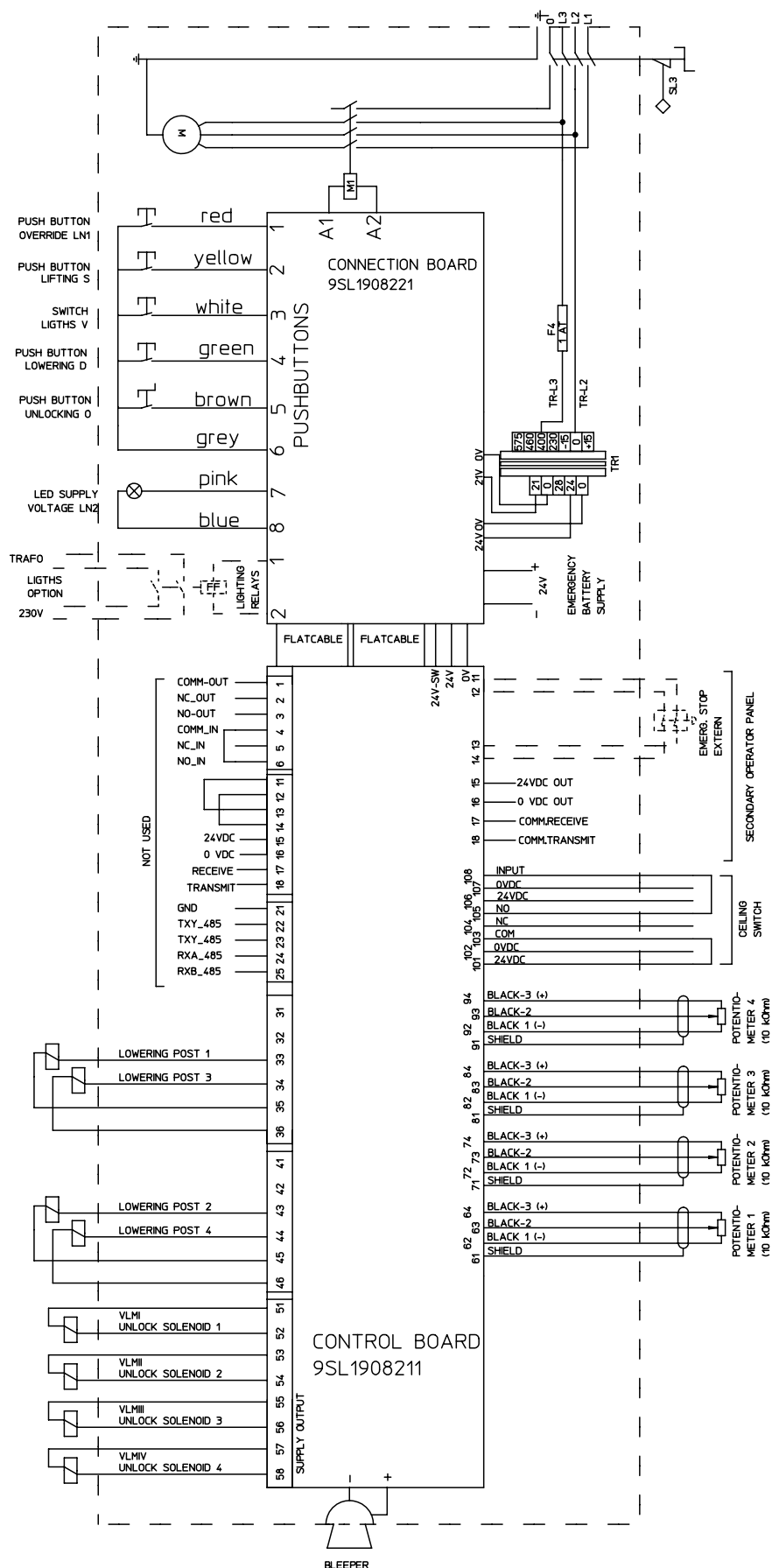
Figure A 7.1 Electric diagram
