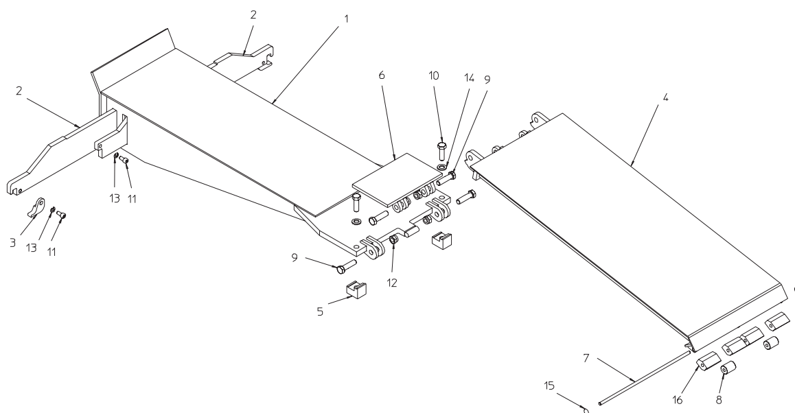
Figure B 3.1 Third track
