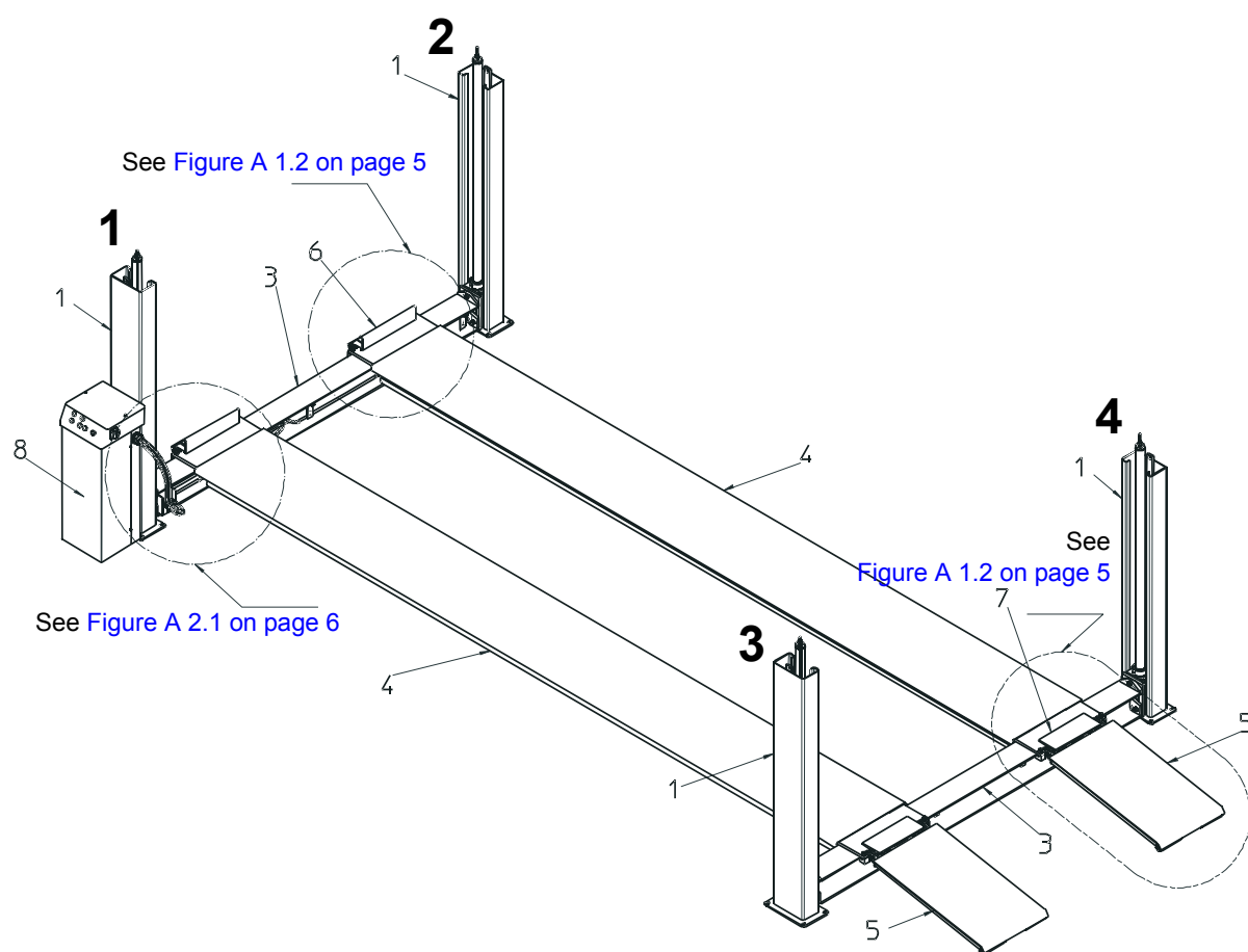
Figure A 1.1 Summary vehicle lift (1)
