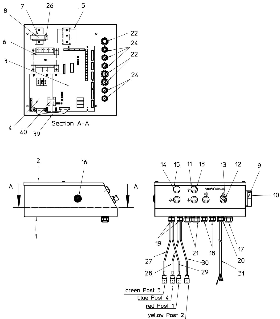
Figure A 7.2 Control box
