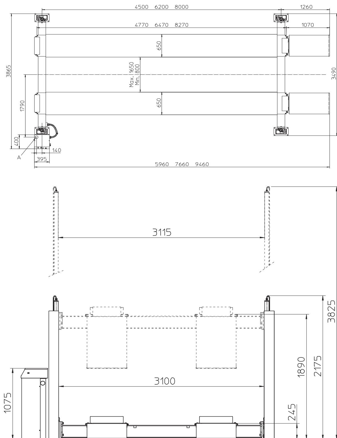
Figure A 9.1 Dimensional drawing
