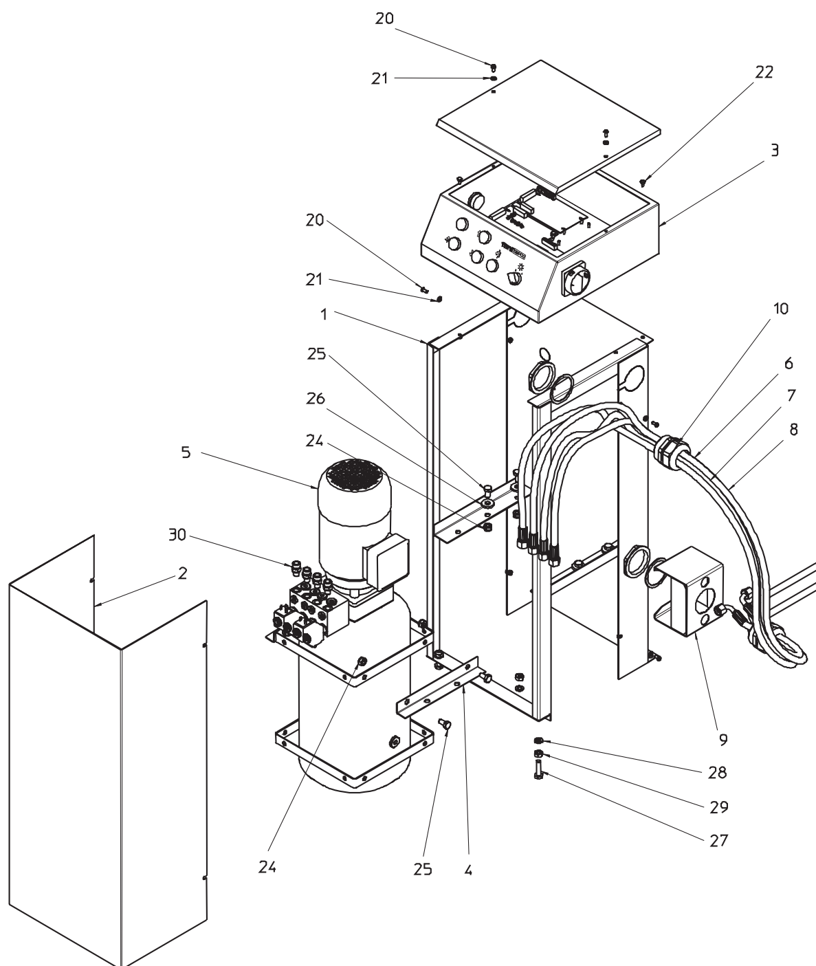
Figure A 3.1 Console
